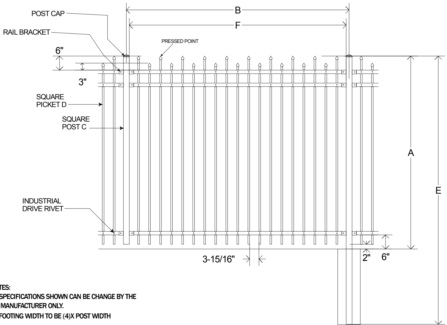
FENCE SECTION ELEVATION
