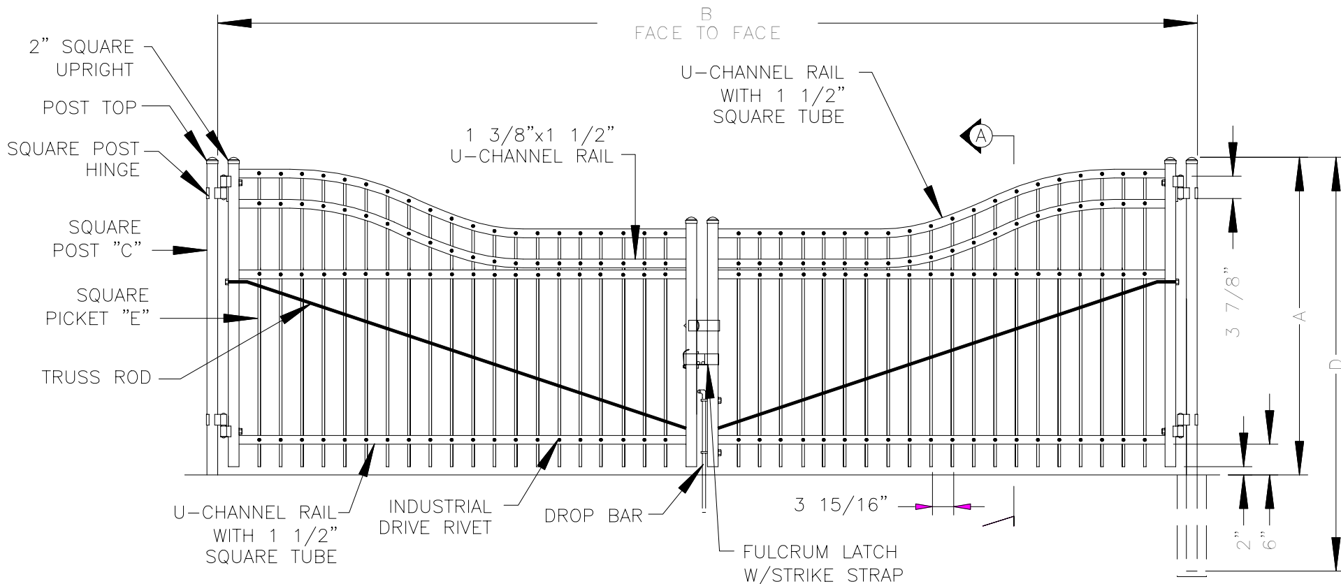
GATE ELEVATION
