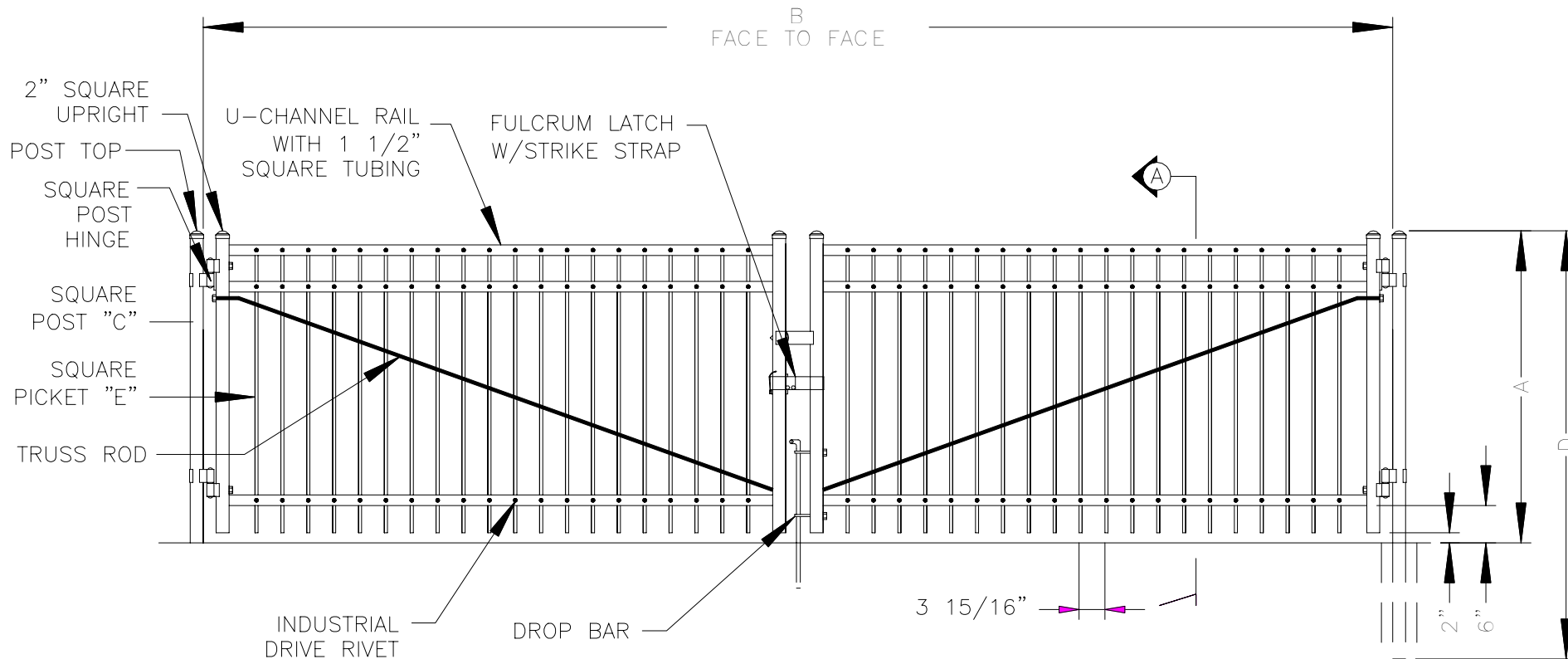
GATE ELEVATION
