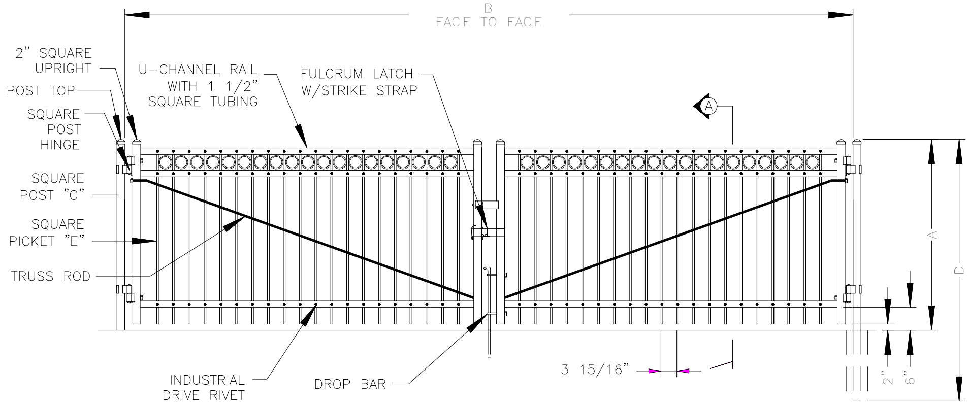
GATE ELEVATION
