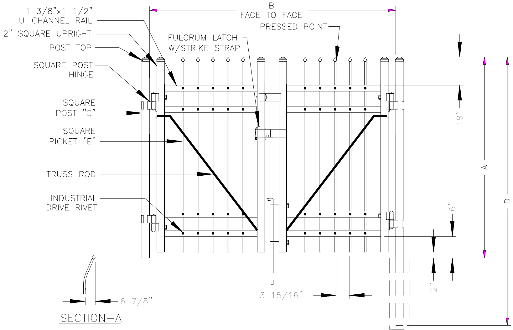
GATE ELEVATION
