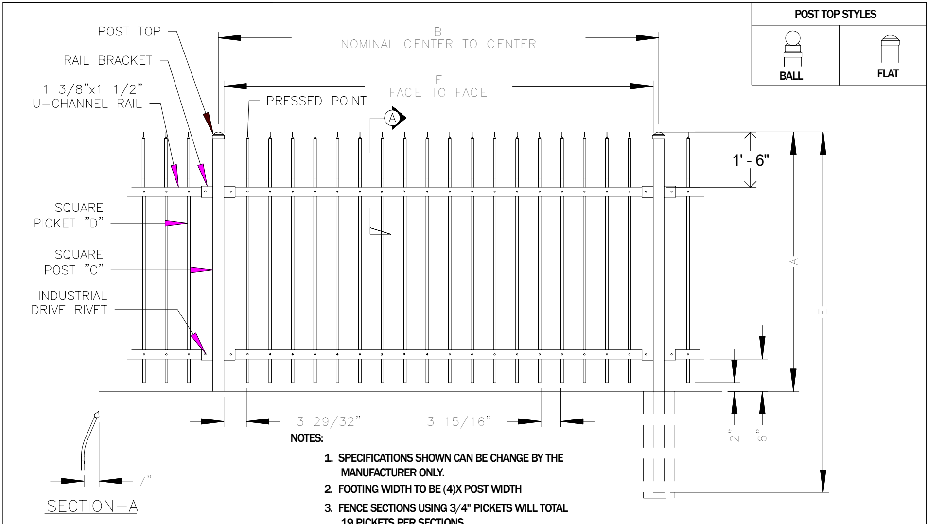
FENCE SECTION ELEVATION
