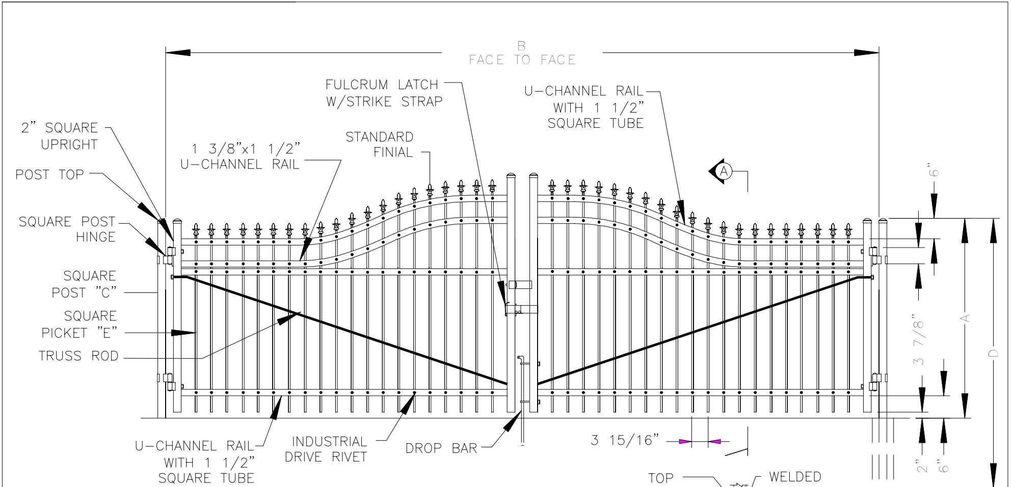
GATE ELEVATION
